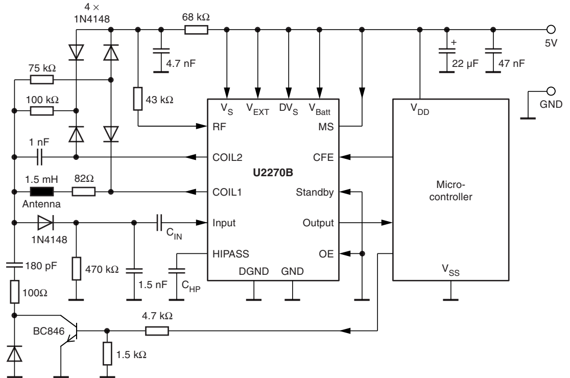
Figure 4-3. Application Circuit 3
